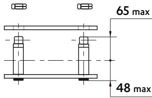
REF N° 209 Connecting link with self-locking nuts
