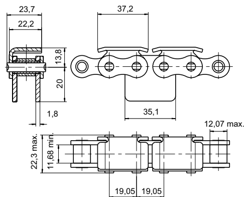
Chain 13N (12B-1) (drawing 5268-27)
