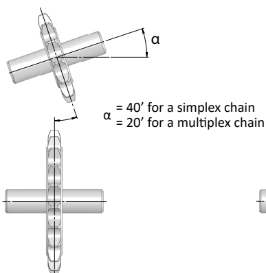
parallelism tolerance
