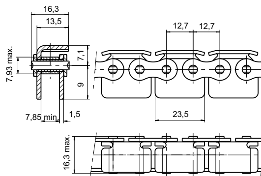
Chain 40-1 (08A-1) (drawing 5415-08)
