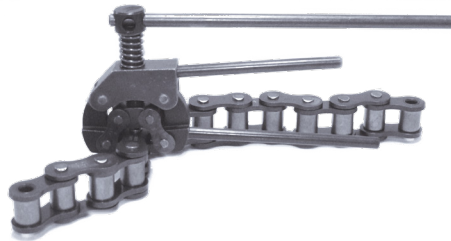
Chain Extractor ref 9160
